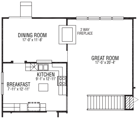
DINING ROOM- GREAT ROOM OPTION
